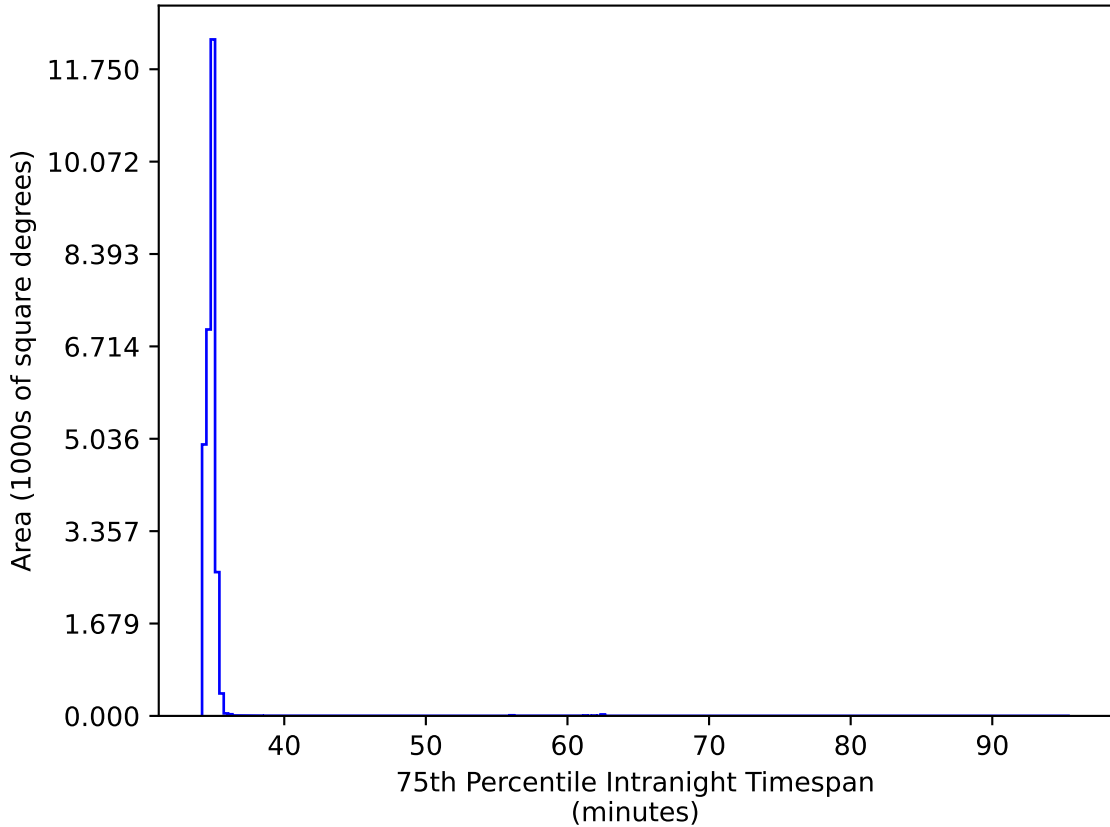
too_ignore_10_4v3.4_10yrs All sky: 75th Percentile Intranight Timespan
