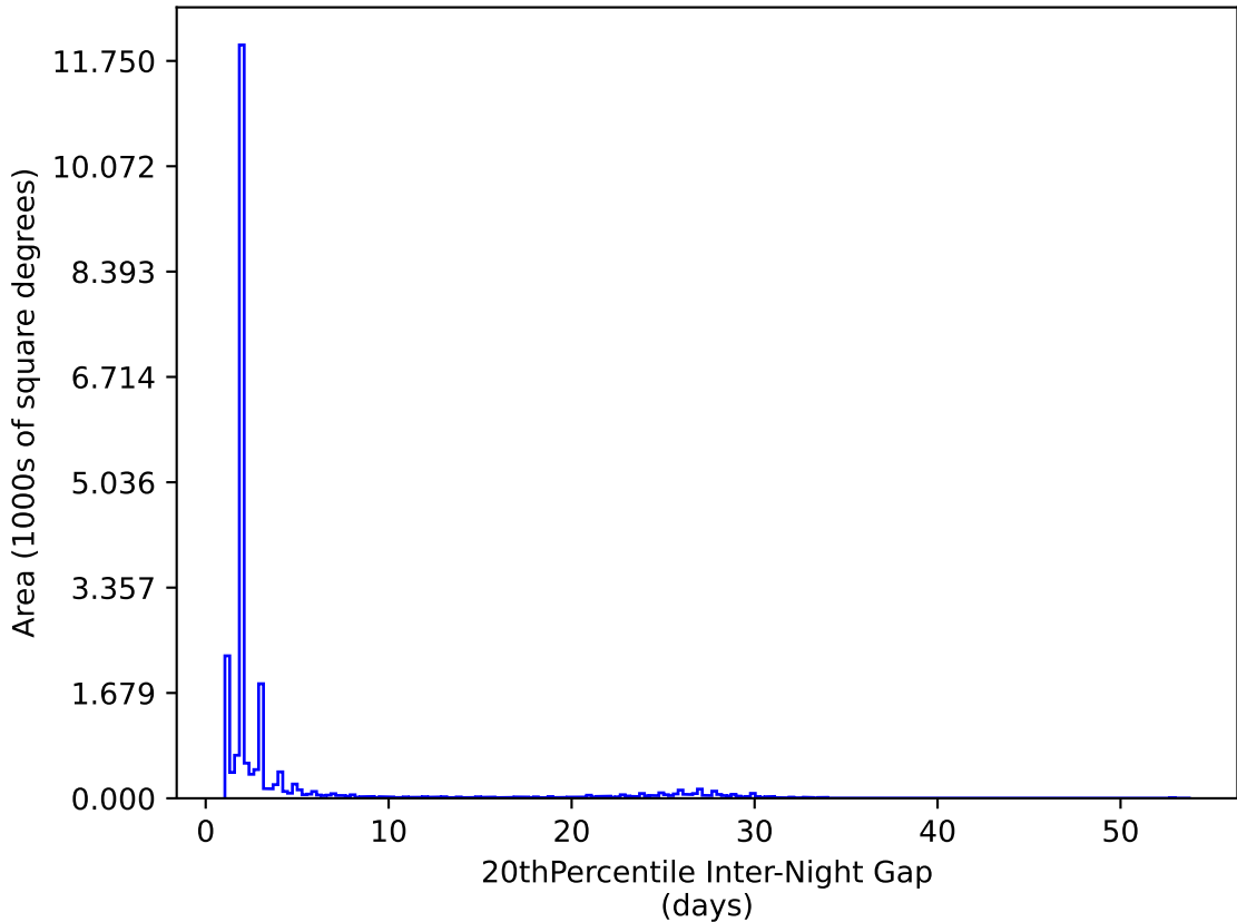
too_ignore_10_4v3.4_10yrs All sky y band: 20thPercentile Inter-Night Gap
