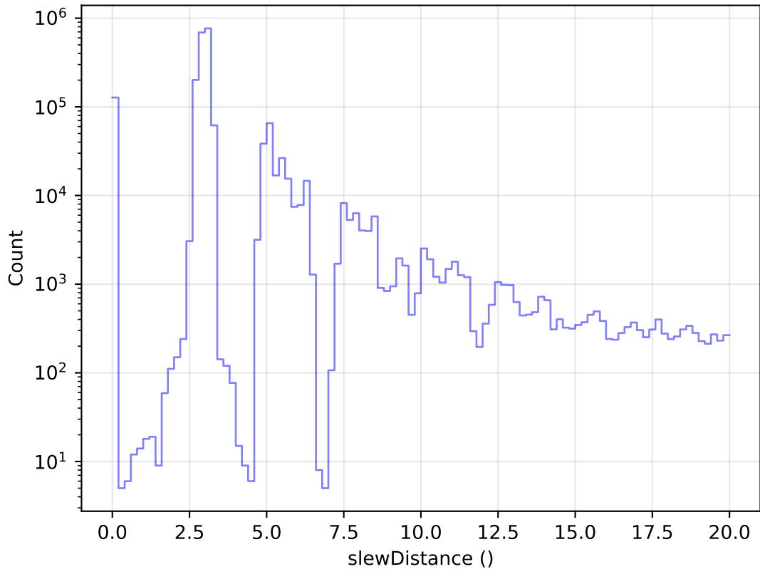
too_ignore_10_4v3.4_10yrs All visits: Zoom Slew Distance Histogram
