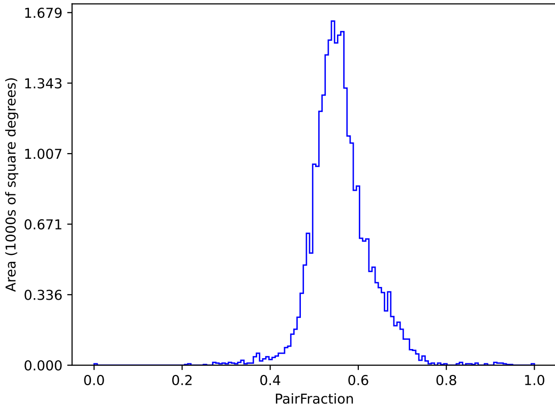
too_ignore_10_4v3.4_10yrs (g or r or i): PairFraction
