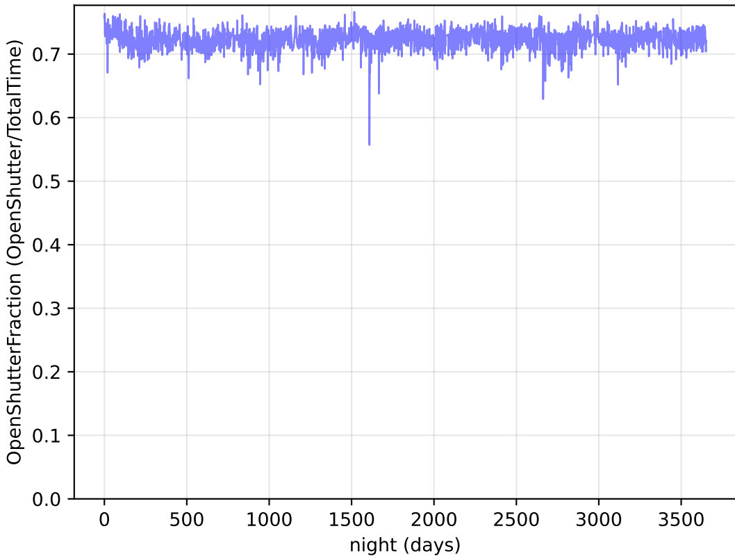
too_ignore_10_4v3.4_10yrs : OpenShutterFraction
