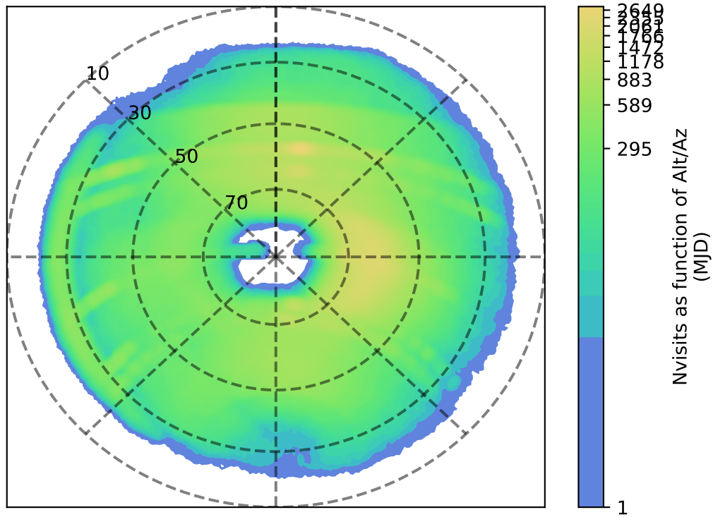
too_ignore_10_4v3.4_10yrs r: Nvisits as function of Alt/Az
