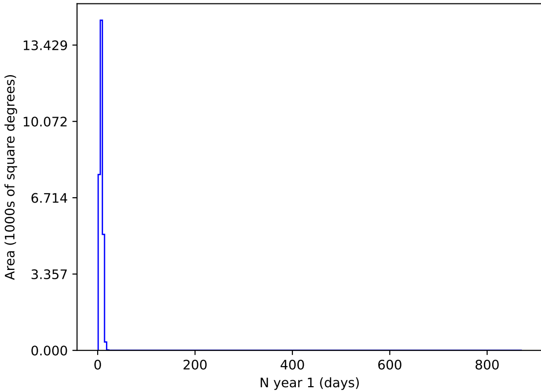
too_ignore_10_4v3.4_10yrs g and night < 365: N year 1
