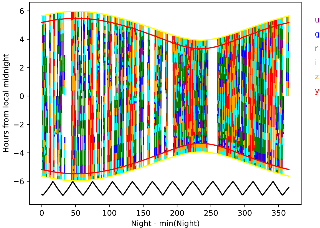
too_ignore_10_4v3.4_10yrs year 5-6: Hourglass
