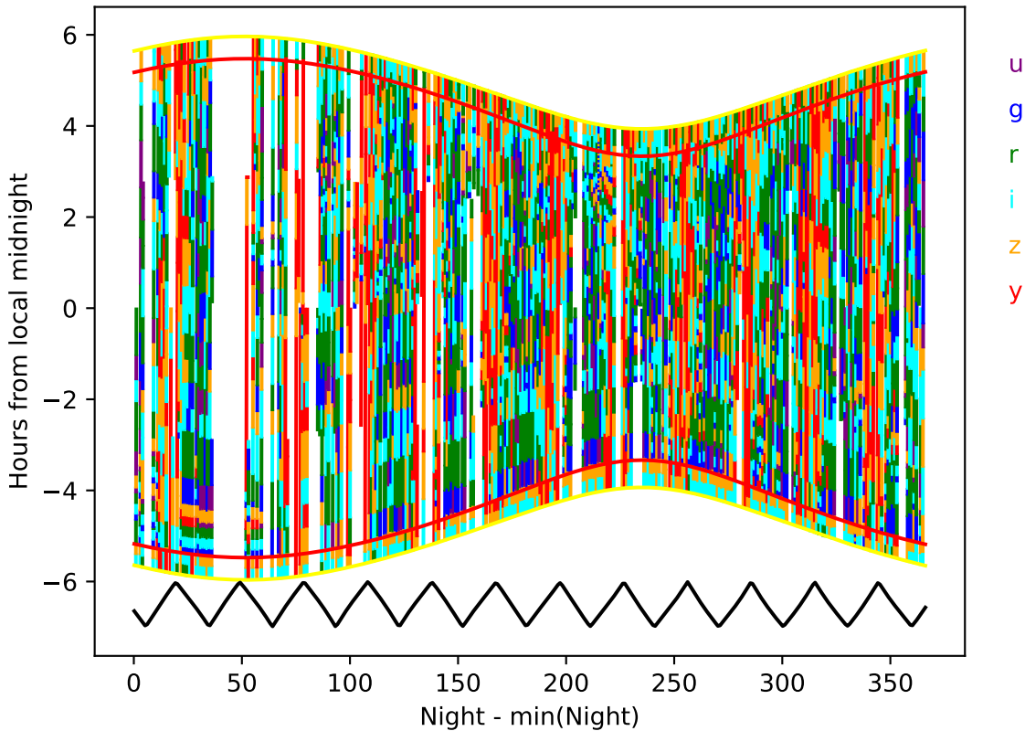
too_ignore_10_4v3.4_10yrs year 2-3: Hourglass
