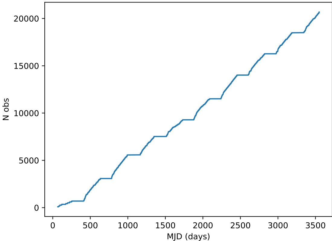
too_ignore_10_4v3.4_10yrs note like DD:ELAISS1%: Cumulative
