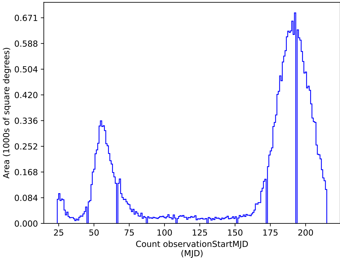
too_ignore_10_4v3.4_10yrs i: Count observationStartMJD
