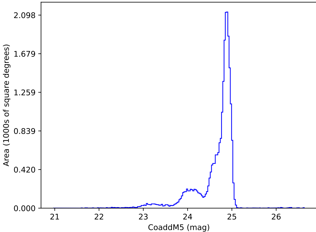
too_ignore_10_4v3.4_10yrs y: CoaddM5
