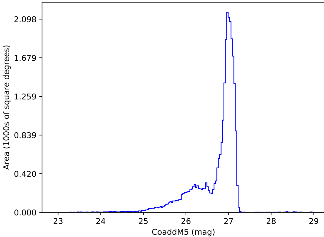
too_ignore_10_4v3.4_10yrs r: CoaddM5
