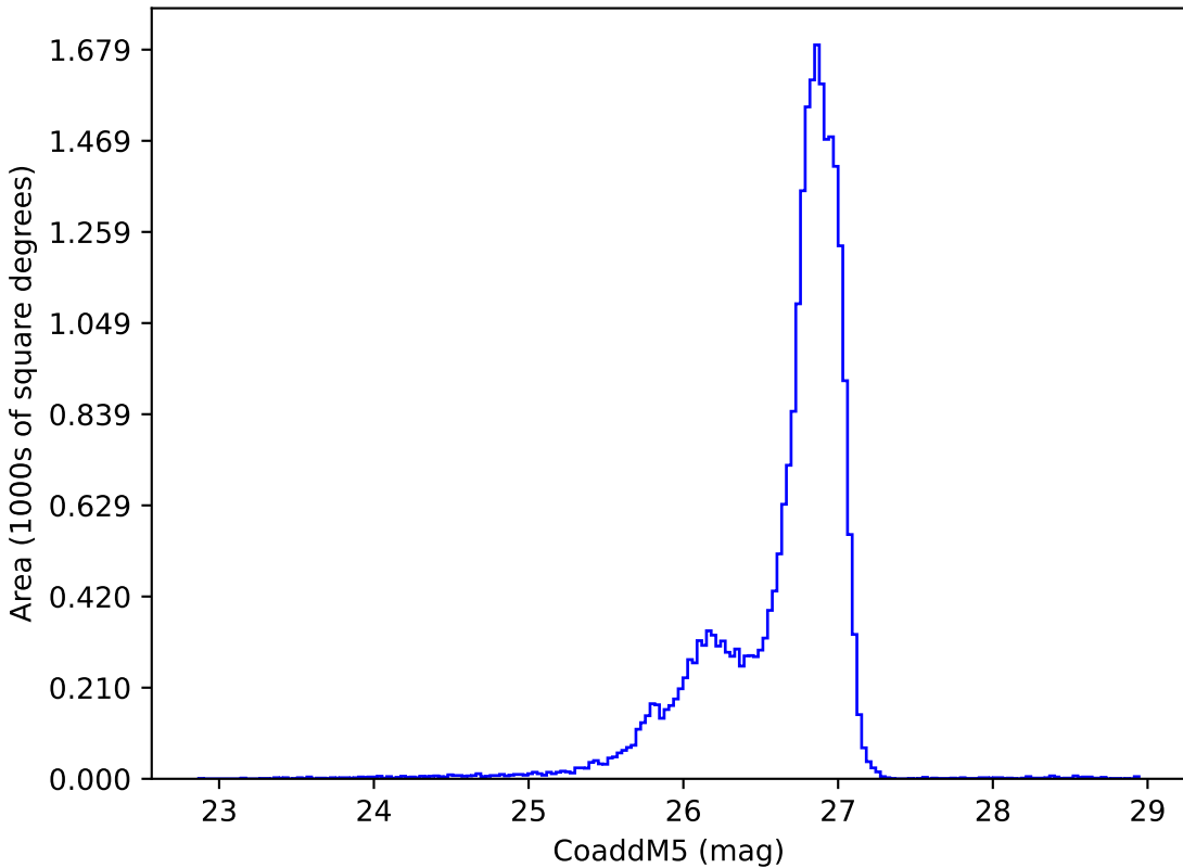
too_ignore_10_4v3.4_10yrs g: CoaddM5
