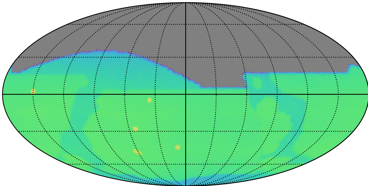
too_ignore_10_4v3.4_10yrs : CoaddM5
