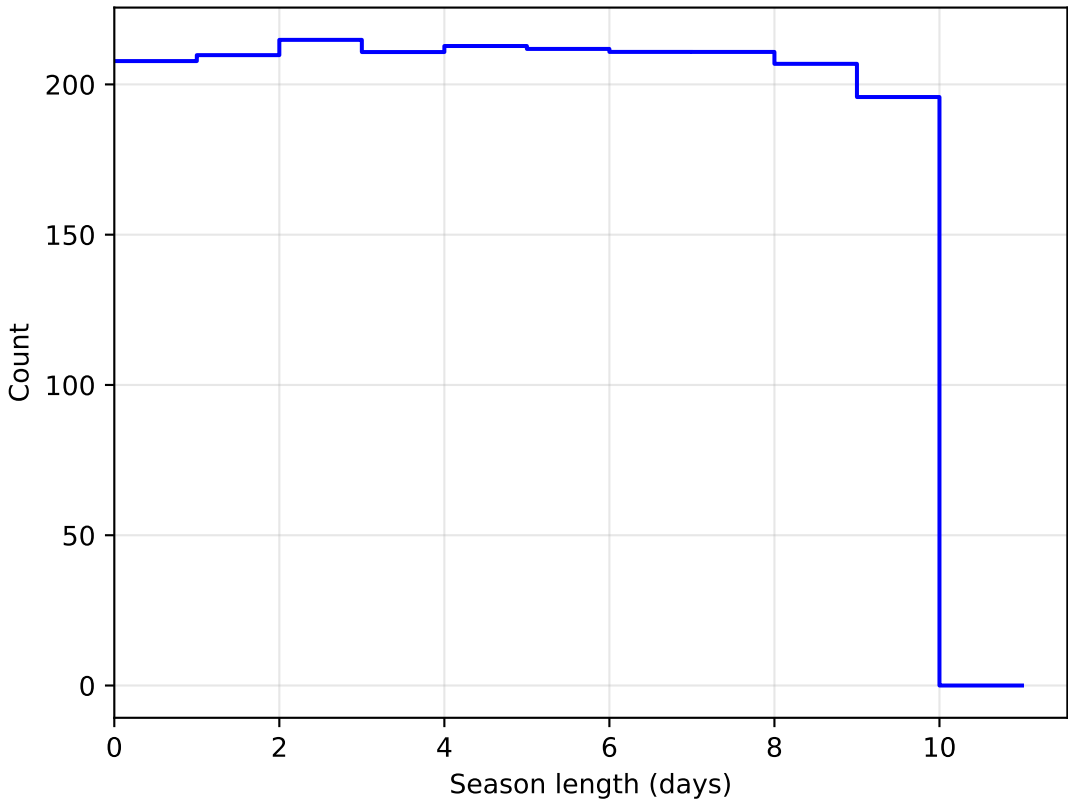
too_ignore_10_4v3.4_10yrs DD:EDFS all bands: SeasonLength
