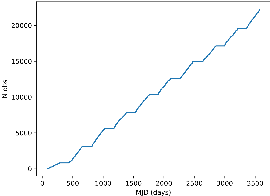
too_ignore_10_4v3.4_10yrs all bands: DD:XMM_LSS Cumulative NVisits
