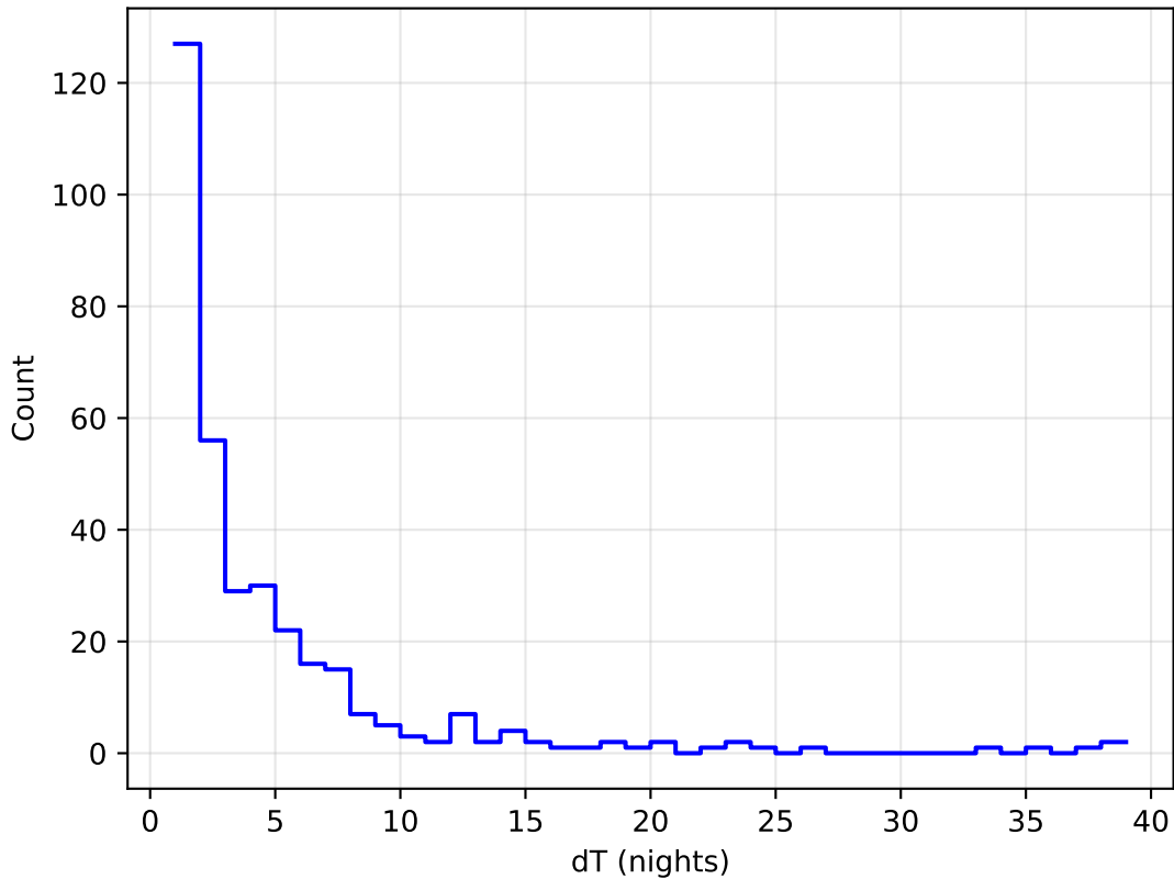
too_ignore_10_4v3.4_10yrs all bands: DD:WFD Delta Nights Histogram
