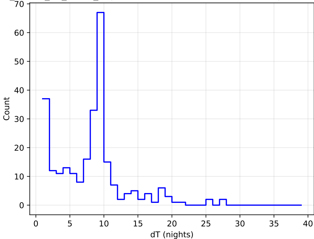
too_ignore_10_4v3.4_10yrs all bands: DD:ELAISS1 Delta Nights Histogram
