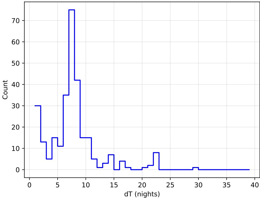
too_ignore_10_4v3.4_10yrs all bands: DD:EDFS Delta Nights Histogram
