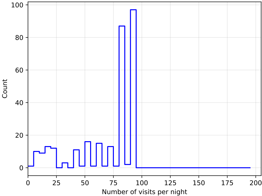
too_ignore_10_4v3.4_10yrs all bands: DD:ECDFS NVisitsPerNight
