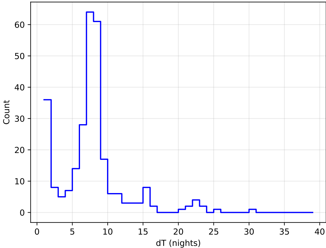
too_ignore_10_4v3.4_10yrs all bands: DD:ECDFS Delta Nights Histogram
