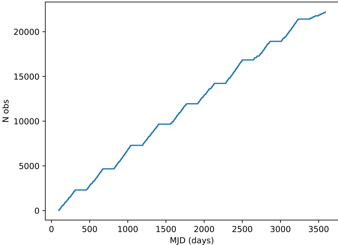
too_ignore_10_4v3.4_10yrs all bands: DD:ECDFS Cumulative NVisits
