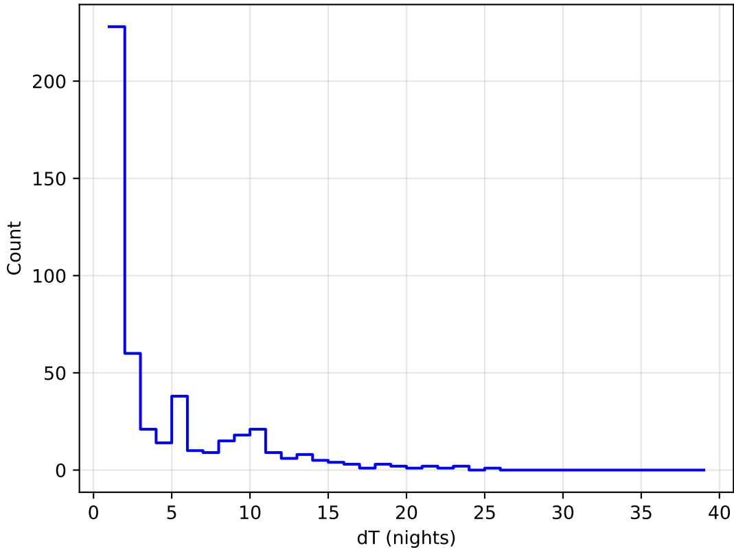
too_ignore_10_4v3.4_10yrs all bands: DD: COSMOS Delta Nights Histogram
