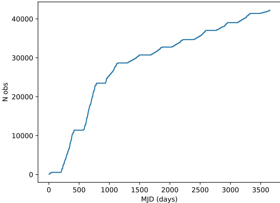
too_ignore_10_4v3.4_10yrs all bands: DD: COSMOS Cumulative NVisits
