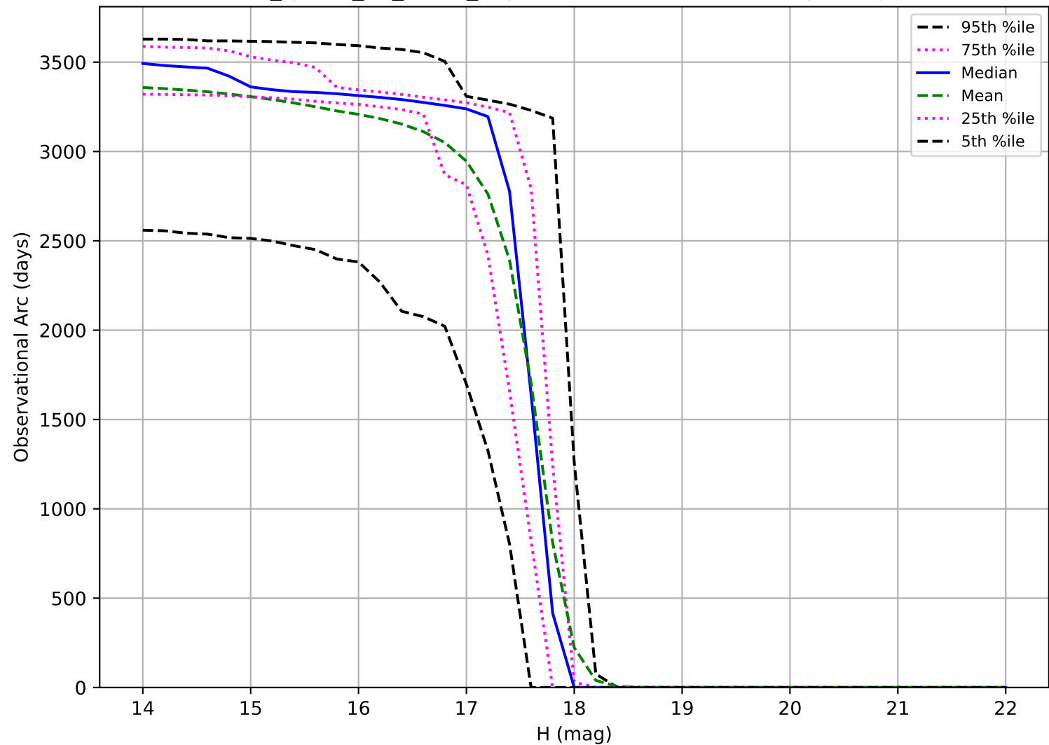
too_ignore_10_1v3.4_10yrs: Observational Arc Length Trojan
