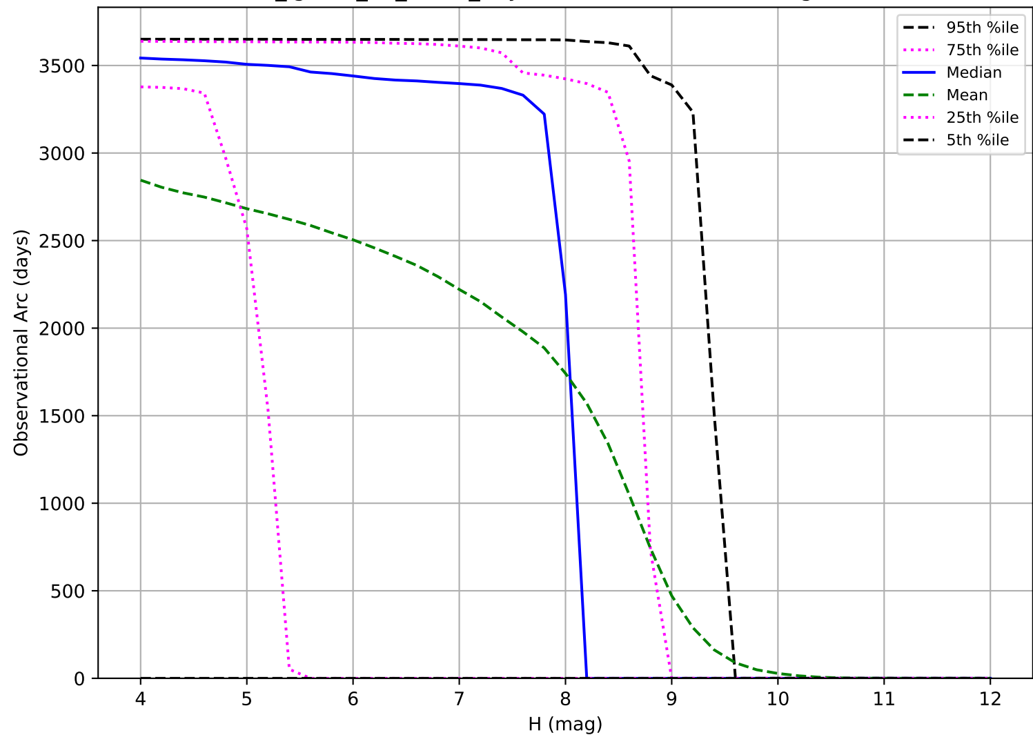
too_ignore_10_1v3.4_10yrs: Observational Arc Length TNO
