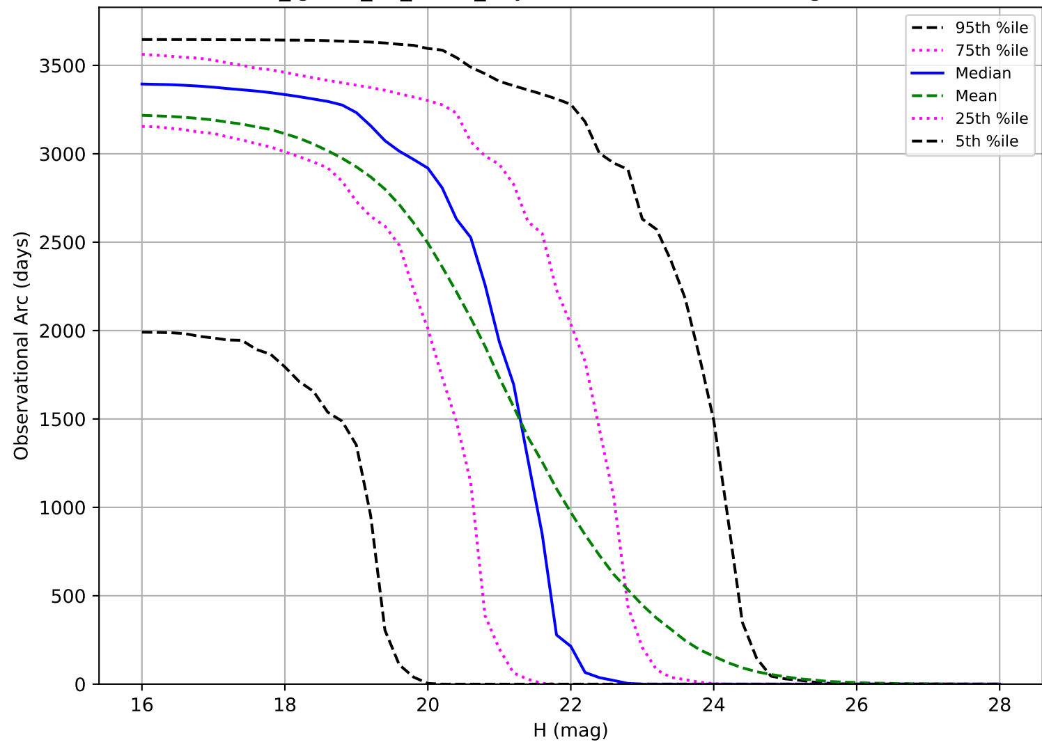
too_ignore_10_1v3.4_10yrs: Observational Arc Length PHA
