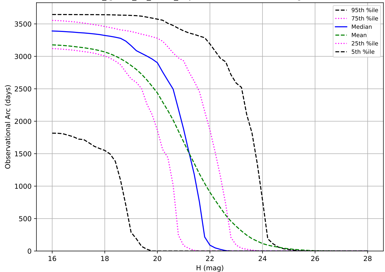
too_ignore_10_1v3.4_10yrs: Observational Arc Length NEO
