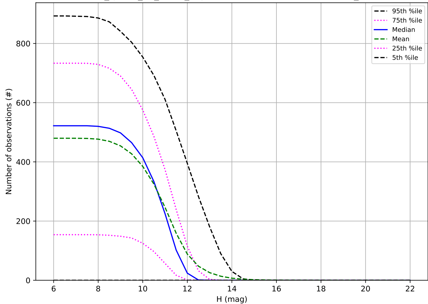
too_ignore_10_1v3.4_10yrs: Number of observations OCC_r20
