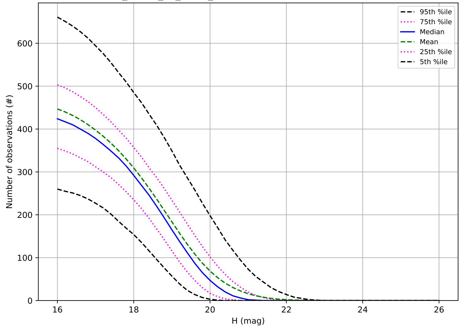
too_ignore_10_1v3.4_10yrs: Number of observations MBA
