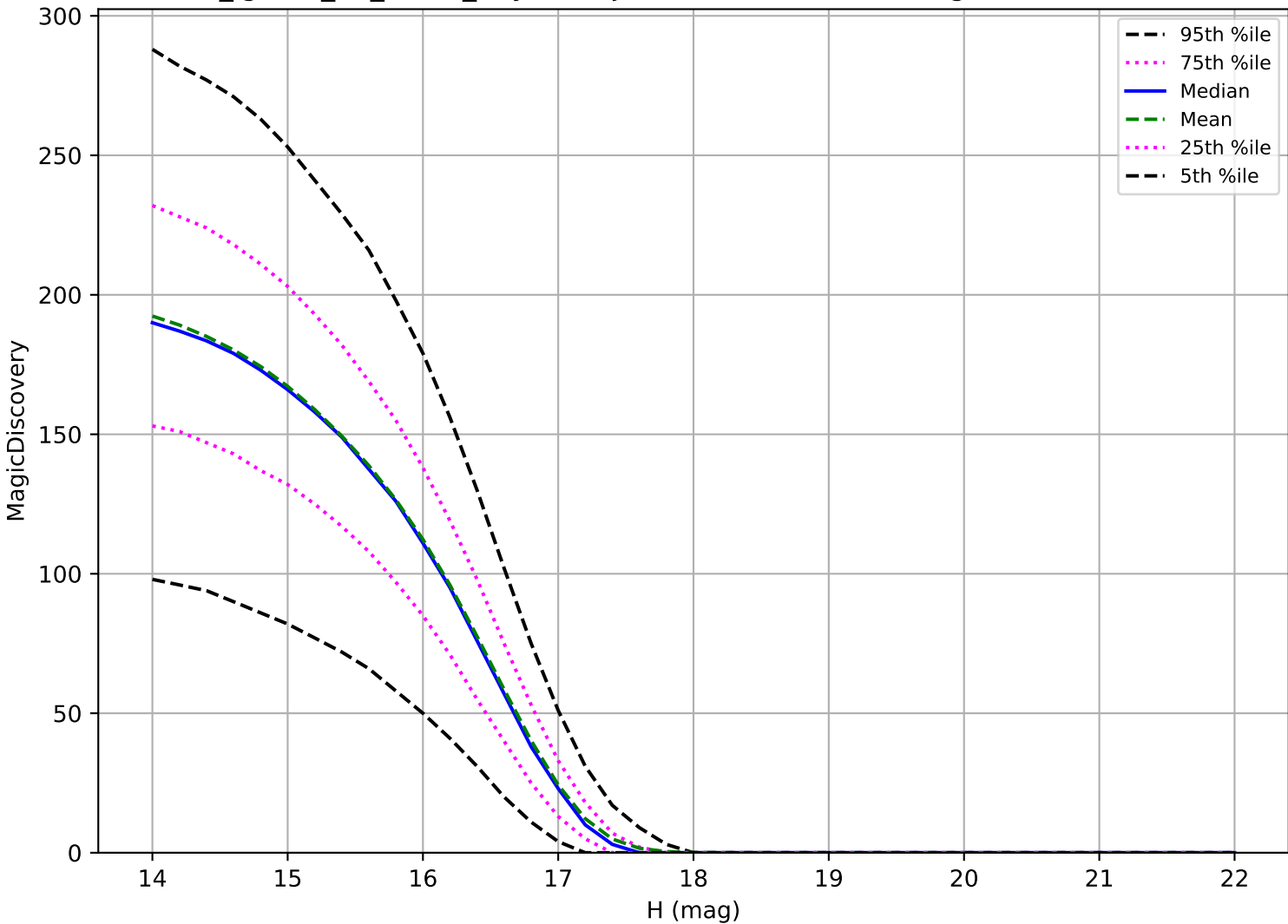
too_ignore_10_1v3.4_10yrs: Trojan 6 detections in 60 nights detection loss
