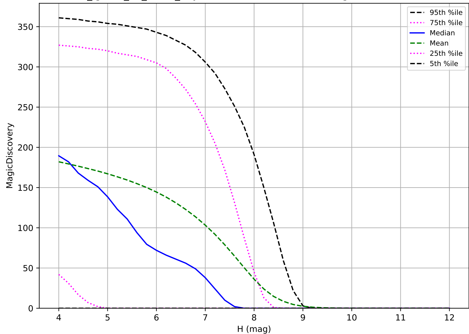
too_ignore_10_1v3.4_10yrs: TNO 6 detections in 60 nights detection loss
