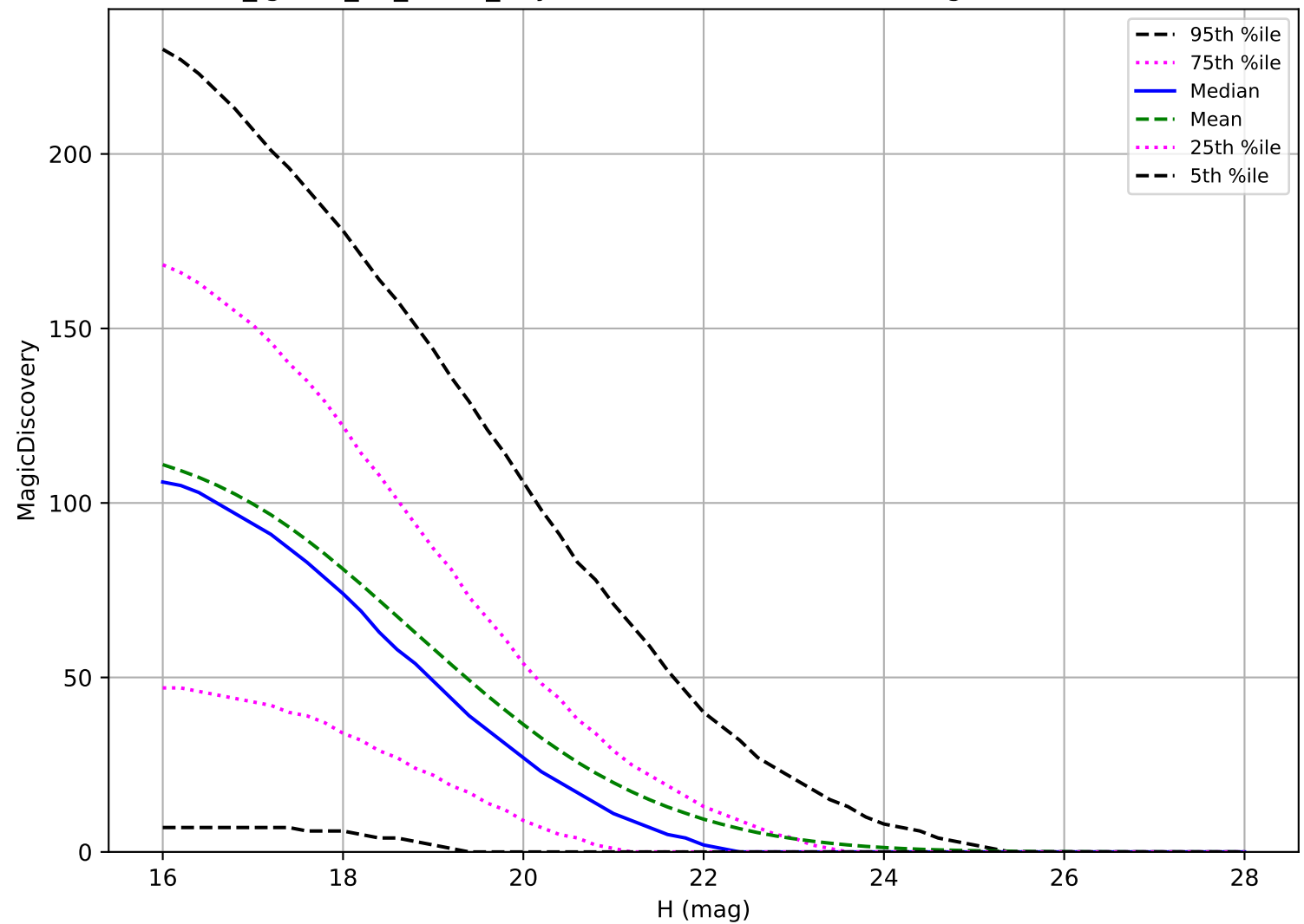
too_ignore_10_1v3.4_10yrs: PHA 6 detections in 60 nights detection loss
