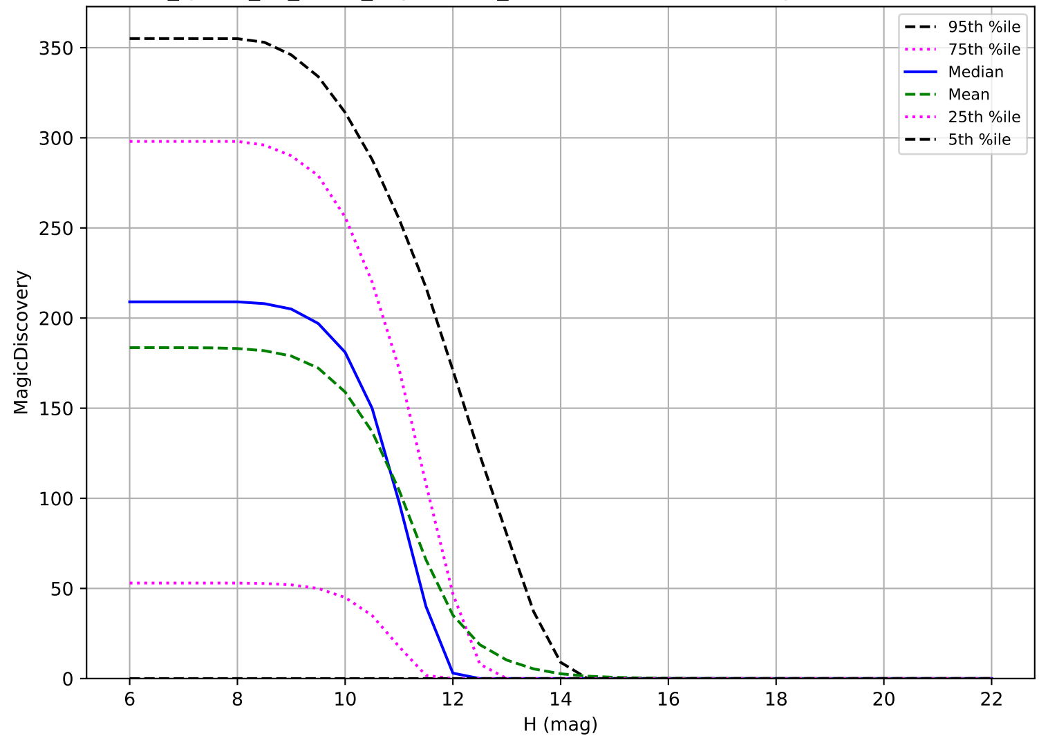
too_ignore_10_1v3.4_10yrs: OCC_r20 6 detections in 60 nights detection loss
