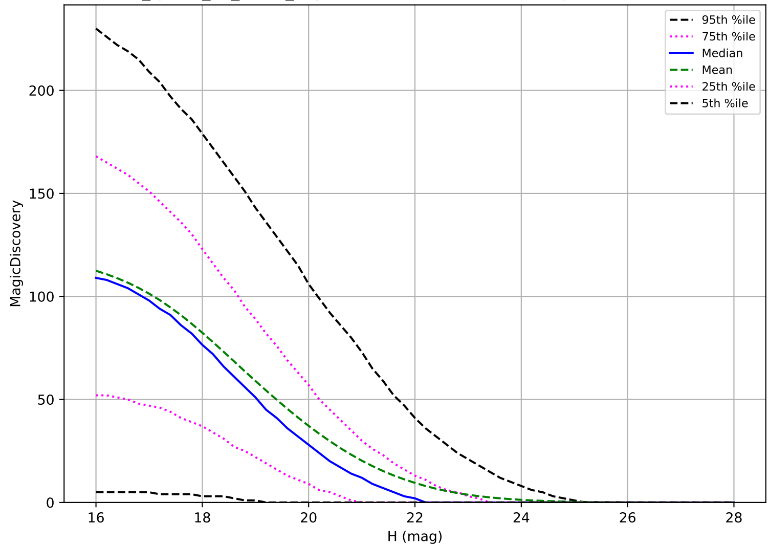
too_ignore_10_1v3.4_10yrs: NEO 6 detections in 60 nights detection loss
