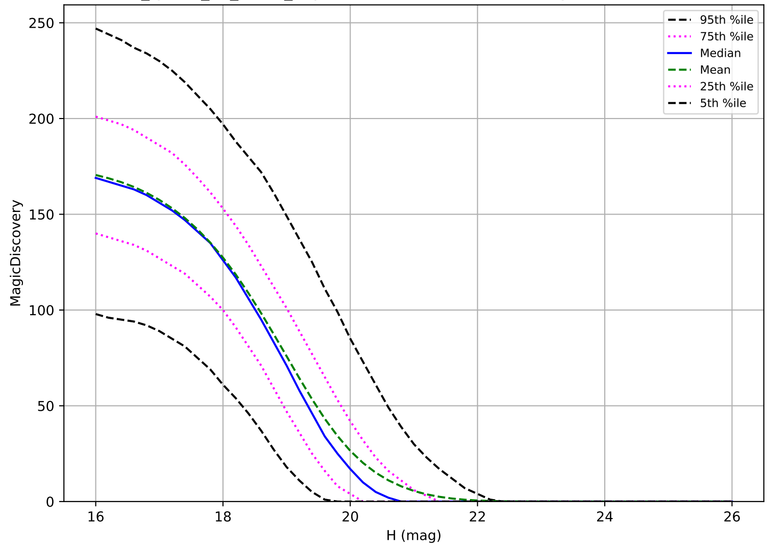
too_ignore_10_1v3.4_10yrs: MBA 6 detections in 60 nights detection loss
