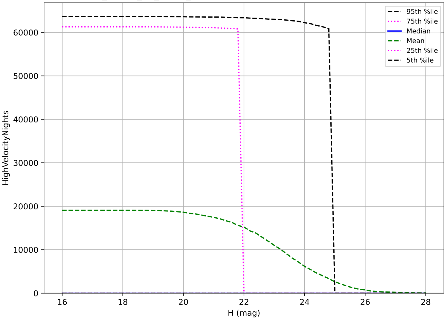
too_ignore_10_1v3.4_10yrs: NEO High velocity pair detection loss
