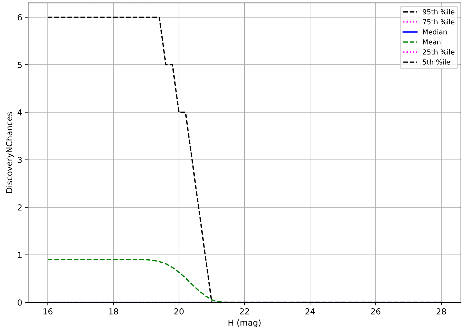
too_ignore_10_1v3.4_10yrs: Vatira 3 pairs in 15 nights detection loss
