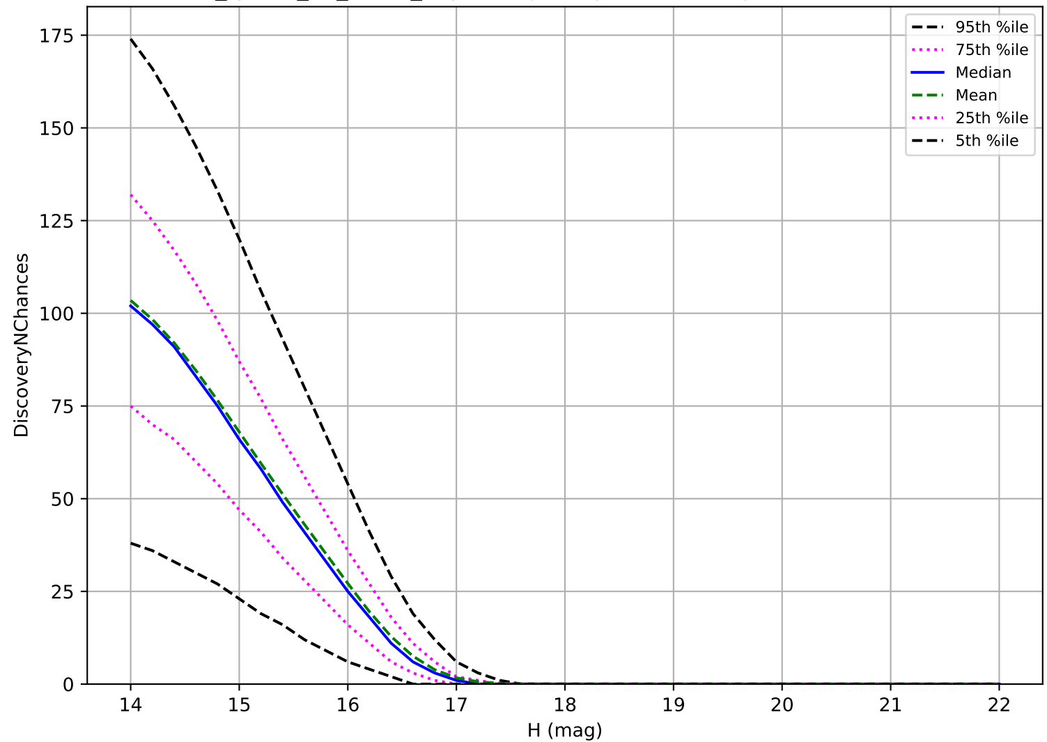
too_ignore_10_1v3.4_10yrs: Trojan 3 pairs in 15 nights detection loss
