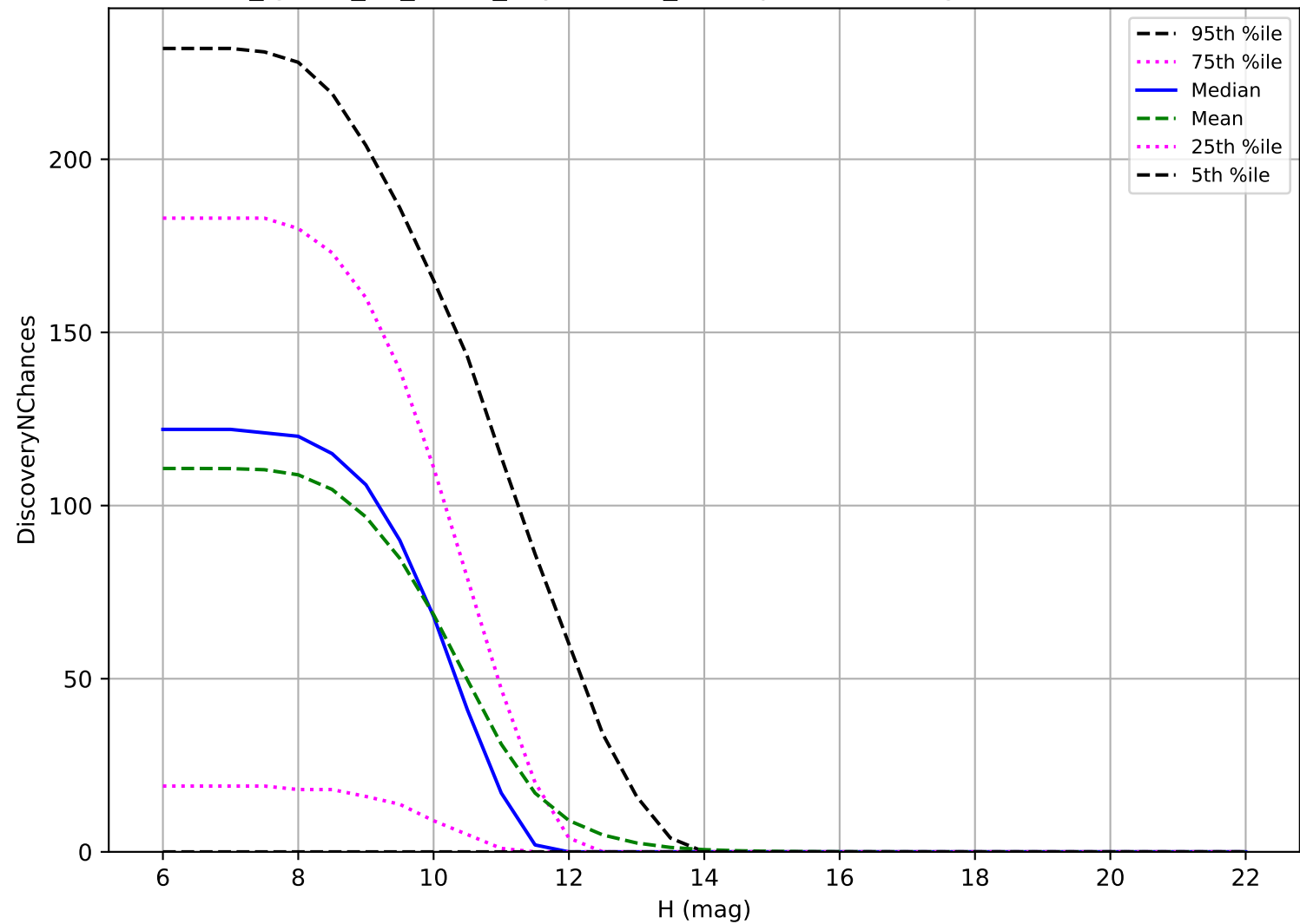
too_ignore_10_1v3.4_10yrs: OCC_r20 3 pairs in 15 nights detection loss
