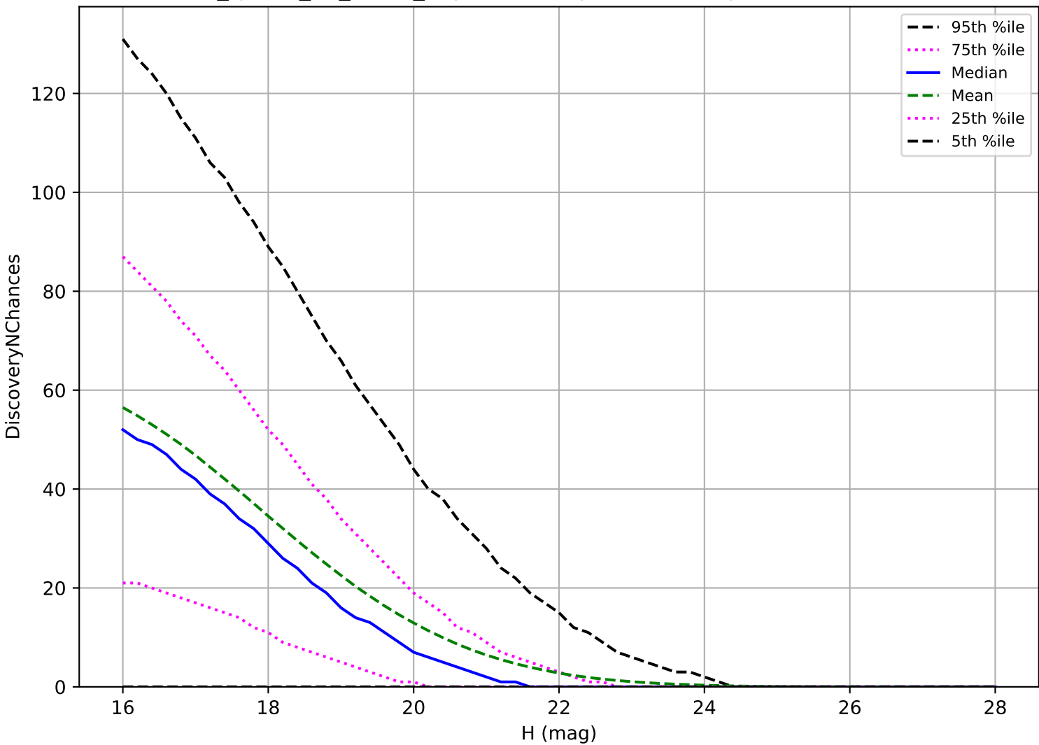
too_ignore_10_1v3.4_10yrs: NEO 3 pairs in 15 nights detection loss
