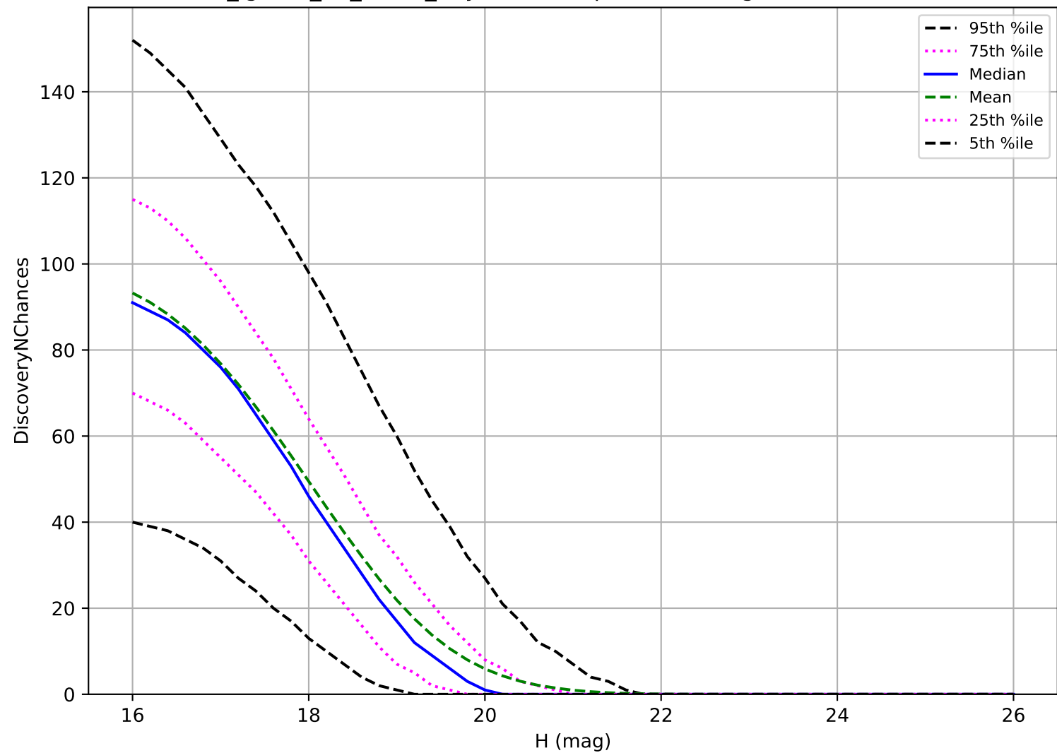
too_ignore_10_1v3.4_10yrs: MBA 3 pairs in 15 nights detection loss
