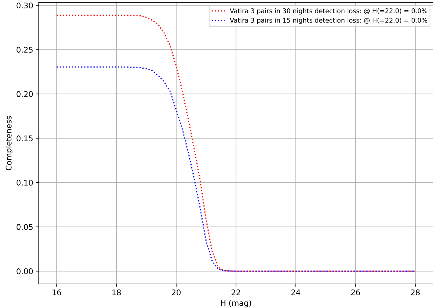
too_ignore_10_1v3.4_10yrs: DifferentialCompleteness
