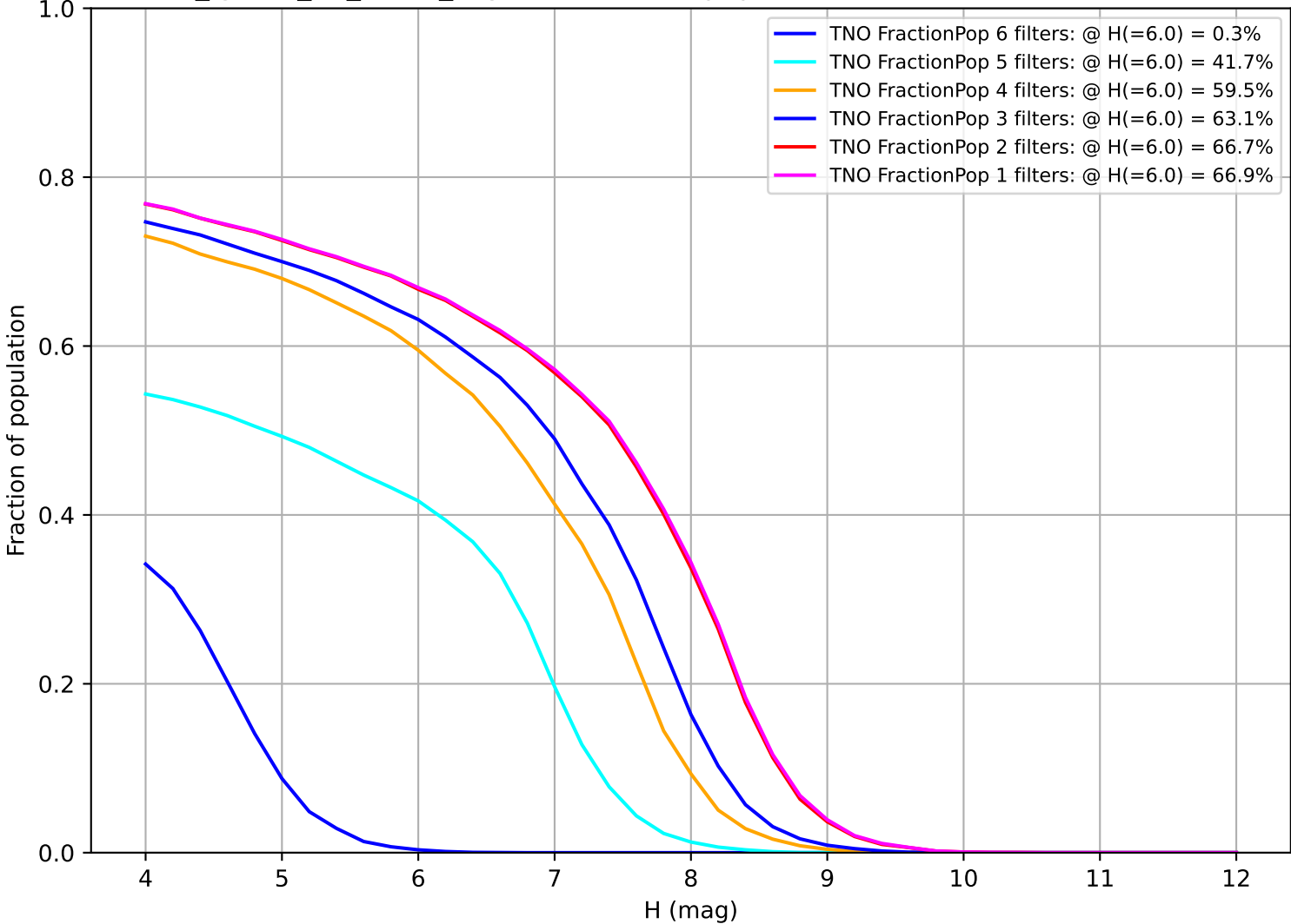
too_ignore_10_1v3.4_10yrs: Fraction of population with colors in X filters TNO
