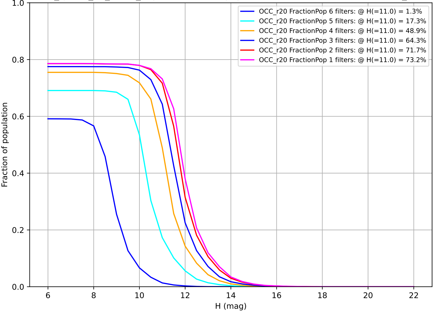
too_ignore_10_1v3.4_10yrs: Fraction of population with colors in X filters OCC_r20
