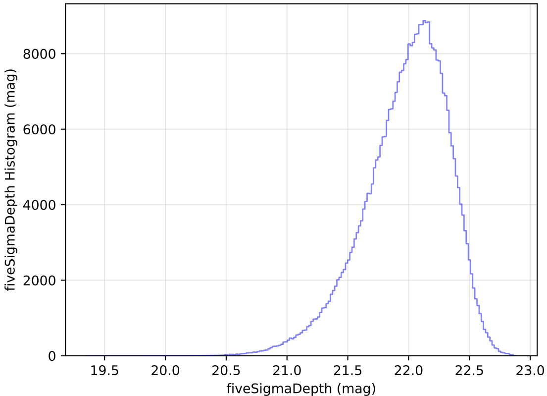
too_ignore_10_1v3.4_10yrs y: fiveSigmaDepth Histogram
