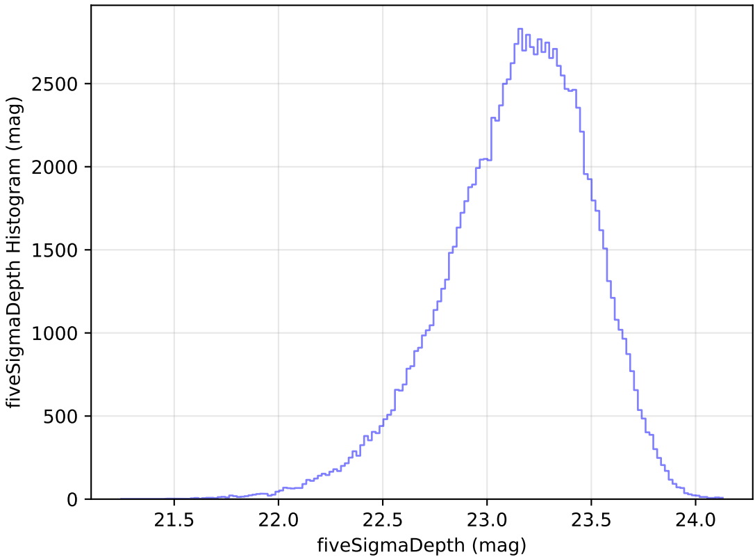
too_ignore_10_1v3.4_10yrs u: fiveSigmaDepth Histogram
