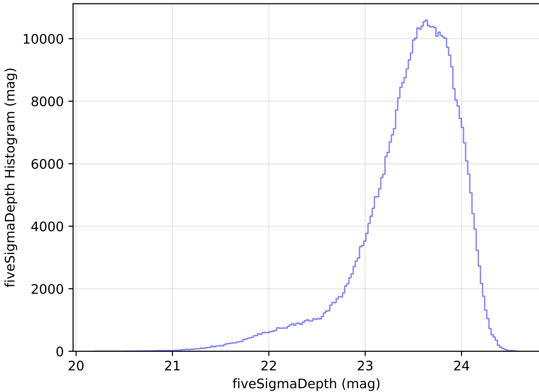
too_ignore_10_1v3.4_10yrs i: fiveSigmaDepth Histogram
