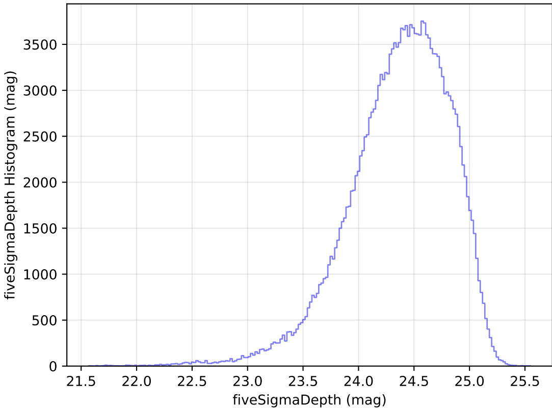
too_ignore_10_1v3.4_10yrs g: fiveSigmaDepth Histogram
